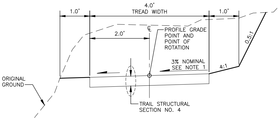
EXCAVATED TRAIL IN ROCK (ET I/R)
