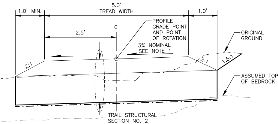
RAISED TRAIL WITH SELECTED MATERIAL (RT W/SM)
