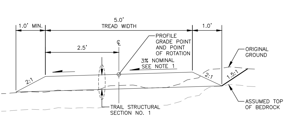
RAISED TRAIL (RT)
