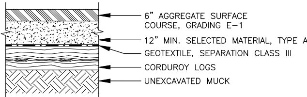
TRAIL STRUCTURAL SECTION NO. 3
