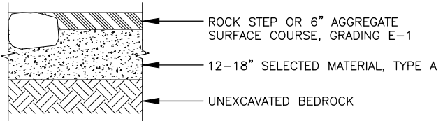
TRAIL STRUCTURAL SECTION NO. 6
