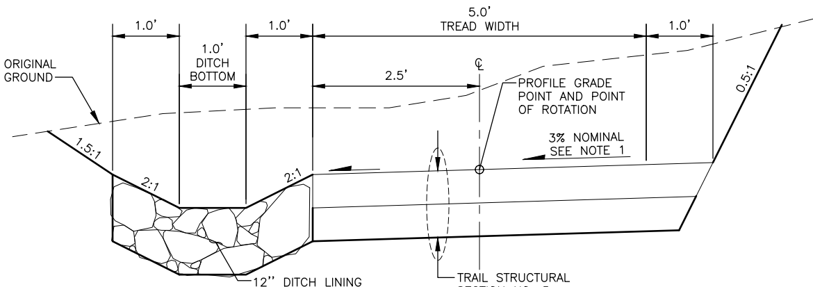
EXCAVATED TRAIL (ET)
