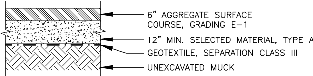
TRAIL STRUCTURAL SECTION NO. 2
