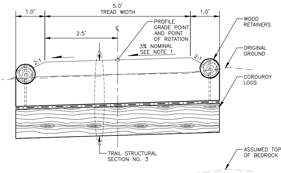
RAISED TRAIL WITH CORDUROY (RT W/C)
